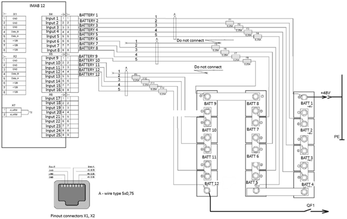
Connection diagram for a 12X4V battery to the IMAB
