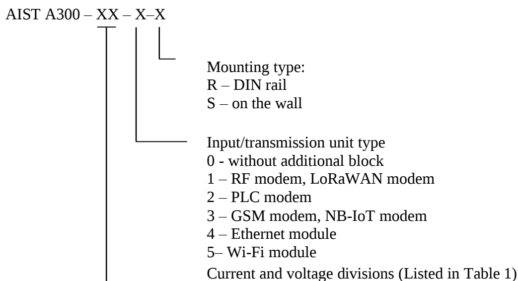
Figure 1 - Structure of the counter symbol
